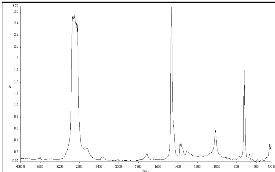
Graph 2: FTIR Spectra of irradiated Polyethylene films containing 1wt% Reverte BD 92771 sample (16473264) for 500 hrs
