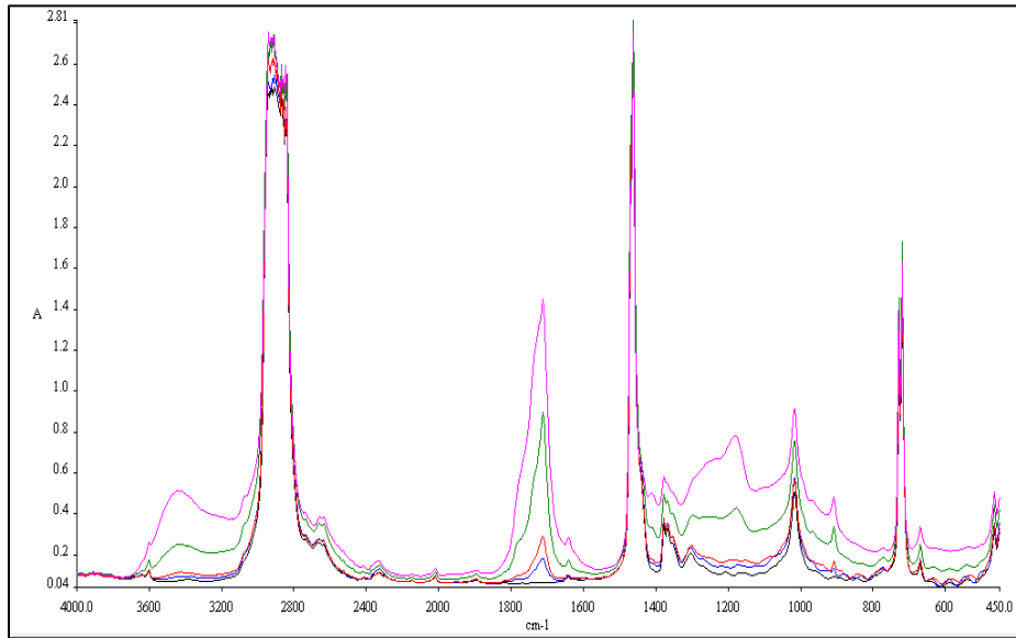
Graph 6: FTIR Spectra overlay of irradiated Polyethylene films containing 1wt% Reverte BD 92771 sample (16473264) initial to 2000 hrs
