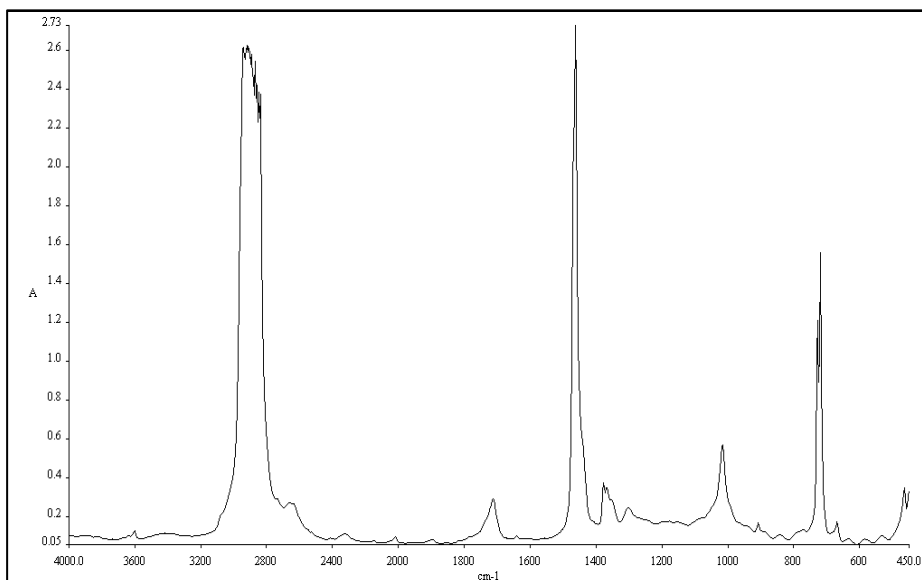
Graph 3: FTIR Spectra of irradiated Polyethylene films containing 1wt% Reverte BD 92771 sample (16473264) for 1000 hrs
