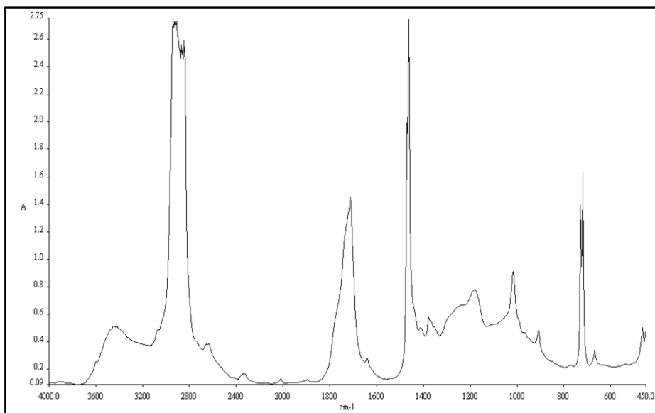
Graph 5: FTIR Spectra of irradiated Polyethylene films containing 1wt% Reverte BD 92771 sample (16473264) for 2000 hrs
