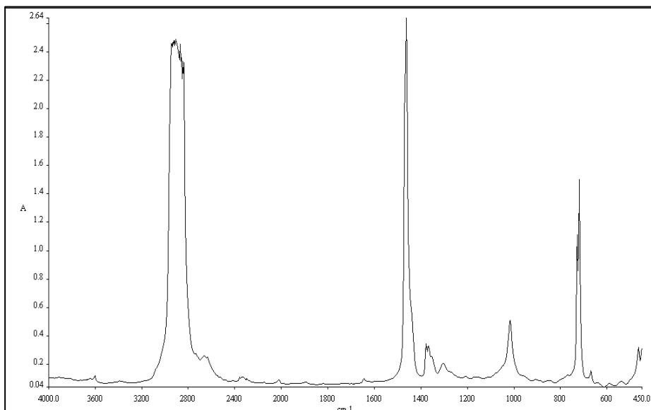
Graph 1: FTIR Spectra of initial unexposed Polyethylene films containing 1wt% Reverte BD 92771 (16473264)
