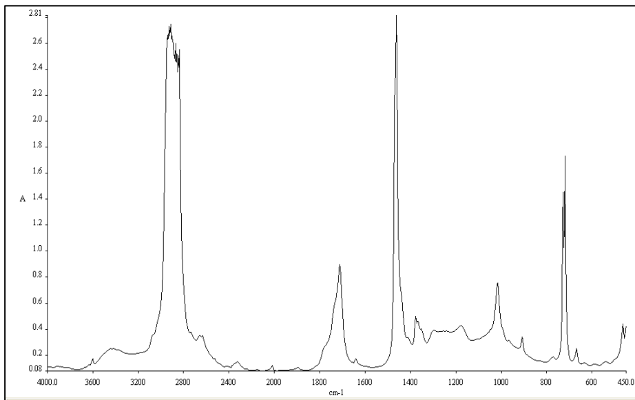
Graph 4: FTIR Spectra of irradiated Polyethylene films containing 1wt% Reverte BD 92771 sample (16473264) for 1500 hrs
